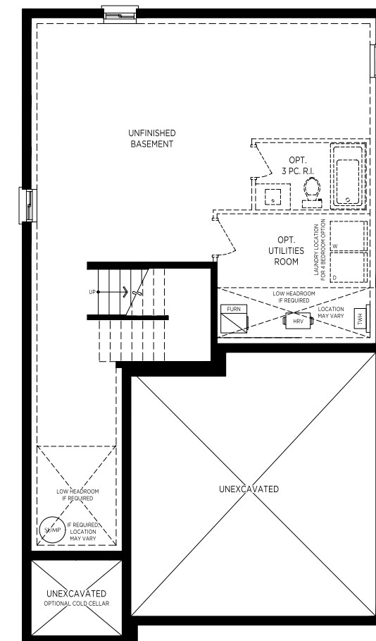
BASEMENT FLOOR PLAN 'A'
