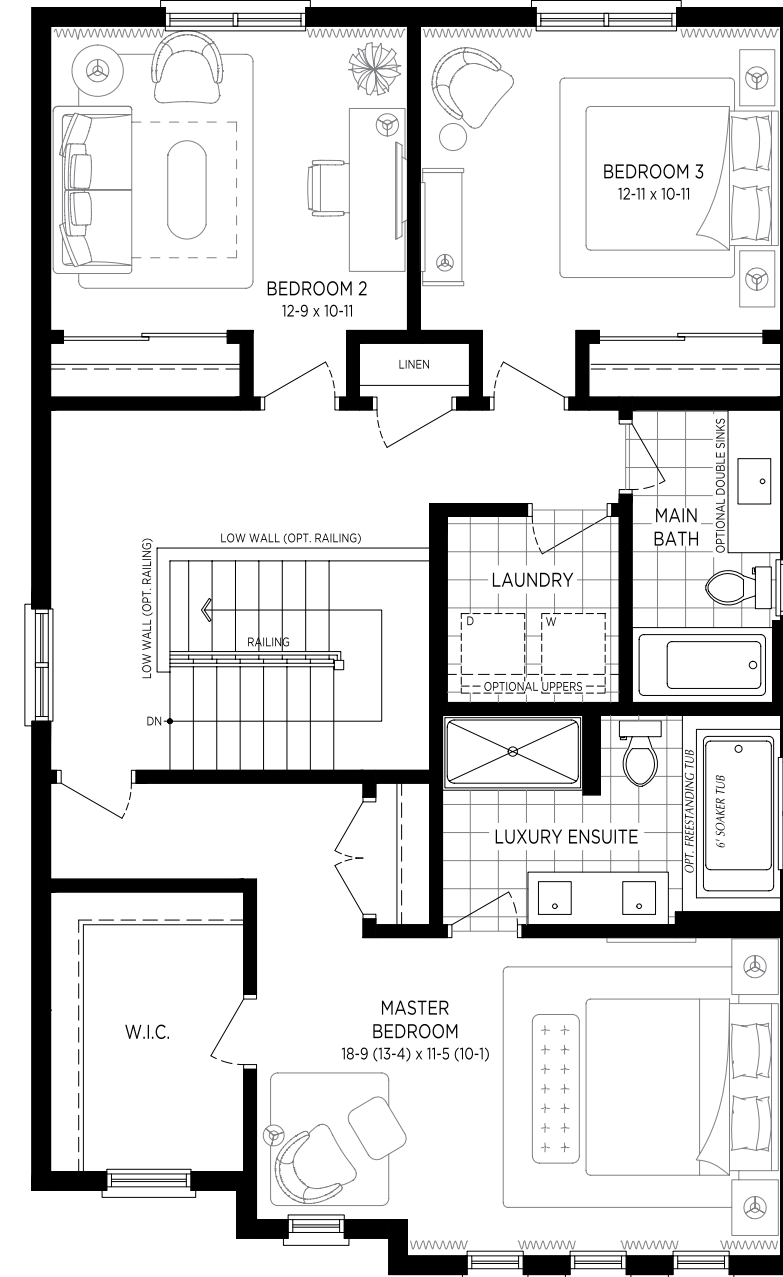
OPT. 1 - SECOND FLOOR PLAN 'A' LUXURY ENSUITE
