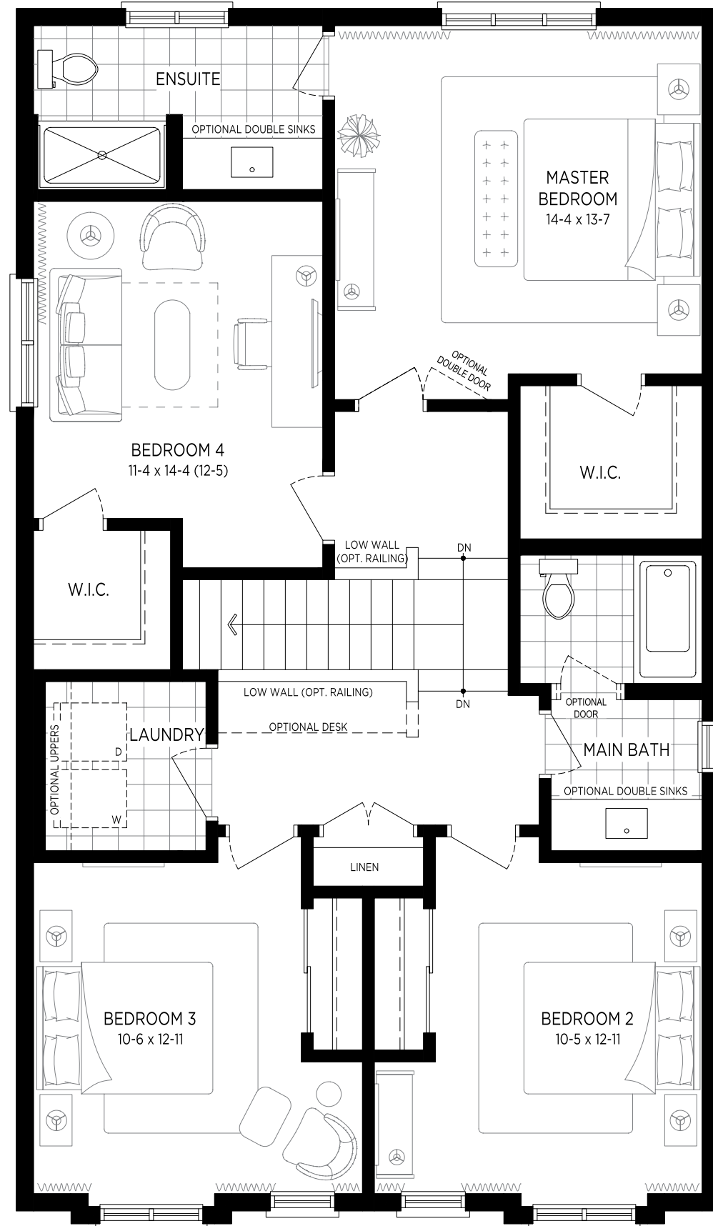
SECOND FLOOR PLAN 'A'
