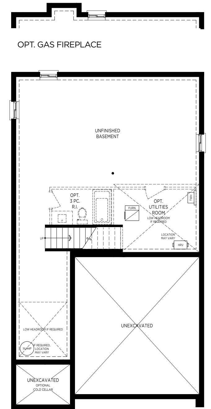
BASEMENT FLOOR PLAN 'A'
