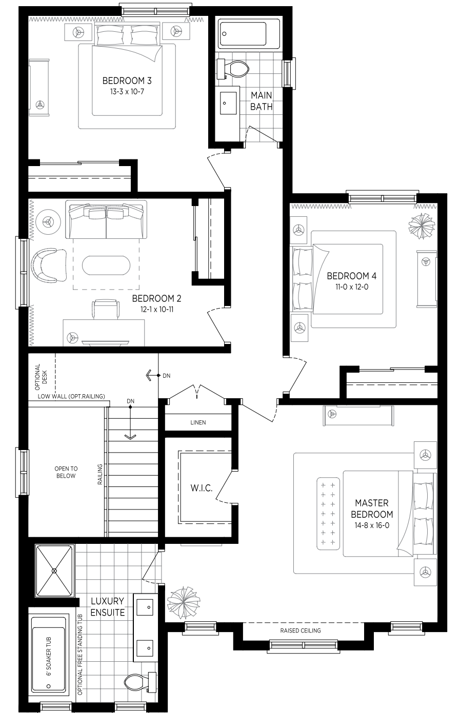
OPT. SECOND FLOOR PLAN 'A' 4 BEDROOM PLAN W/LUXURY ENSUITE
